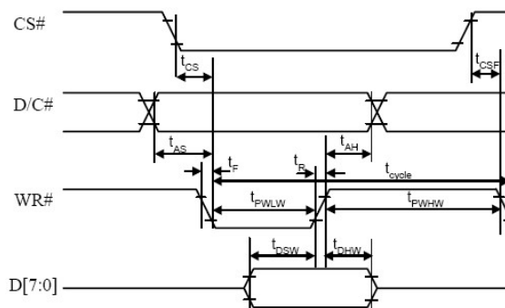
( Write Timing )
