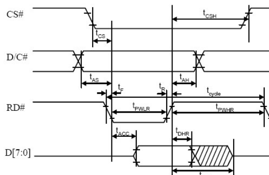
( Read Timing )
